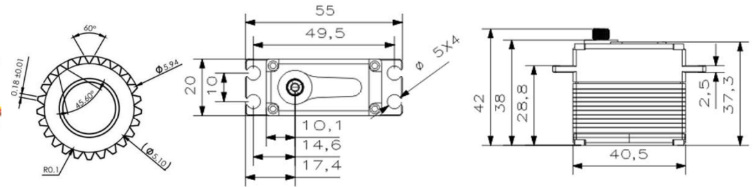
25T 6mm Output Shaft Spline
